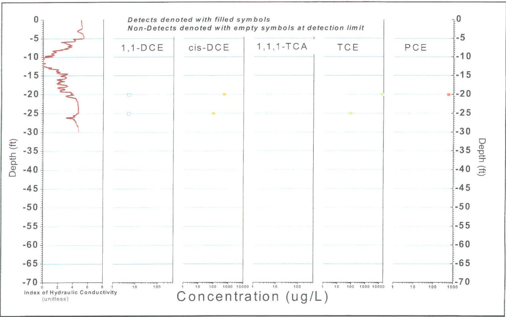
FIGURE B241, I k RECORD AND SELECTED VOC ANALYTICAL RESULTS ERM, Wayland, Massachusetts
