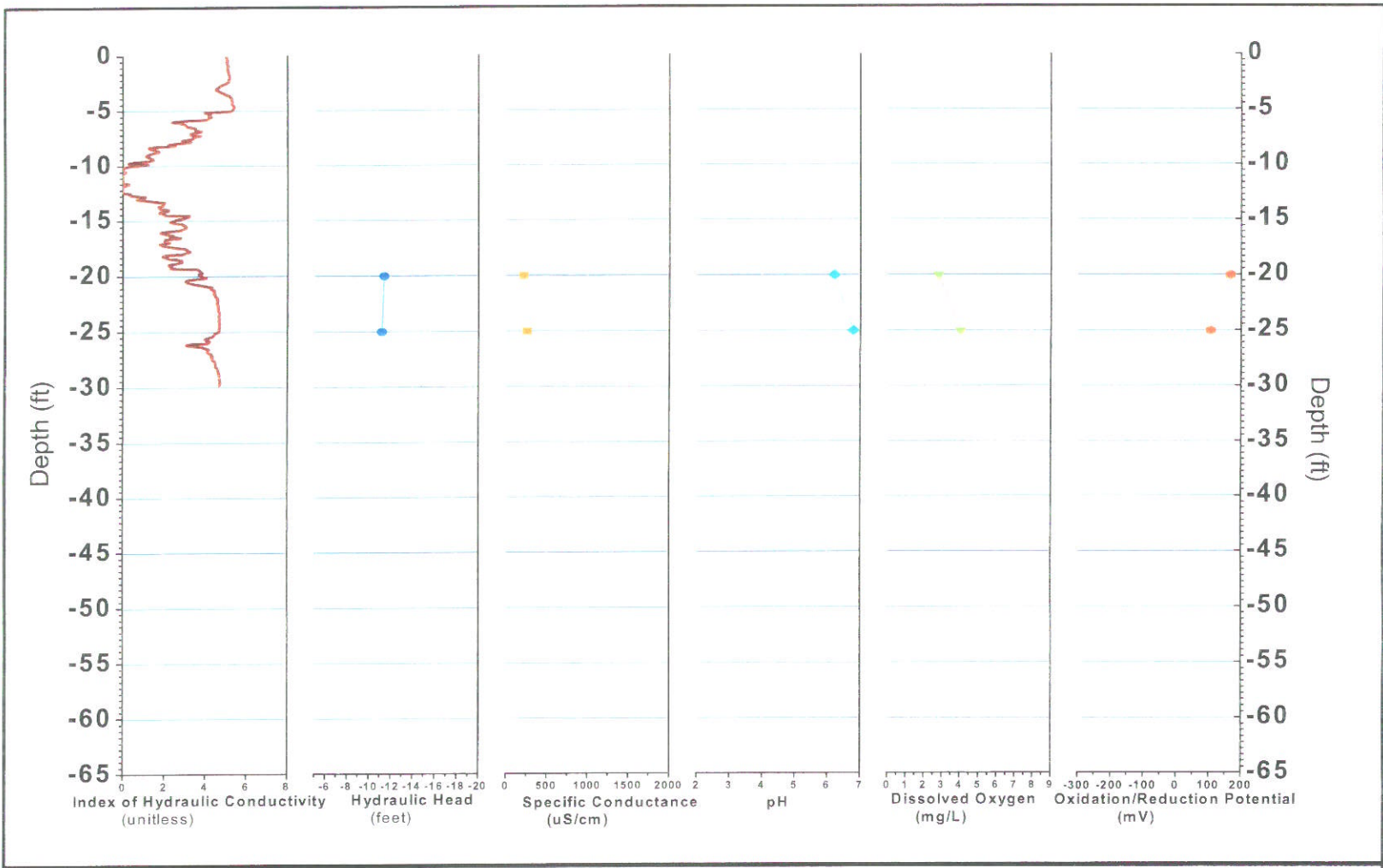
FIGURE B-241, I_k RECORD AND PHYSICO-CHEMICAL PARAMETERS ERM, Wayland, Massachusetts
