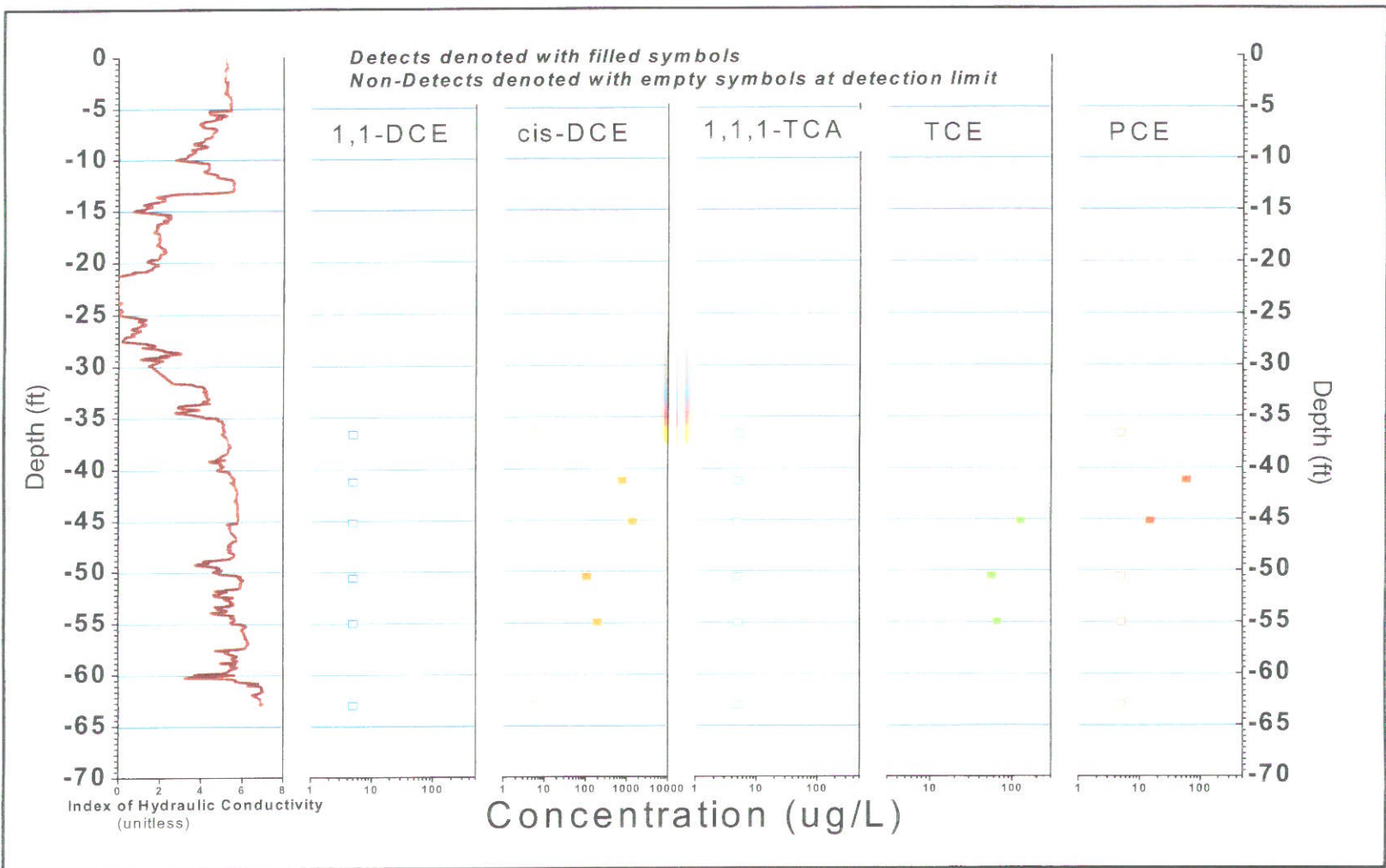
FIGURE B240, I_k RECORD AND SELECTED VOC ANALYTICAL RESULTS ERM, Wayland, Massachusetts
