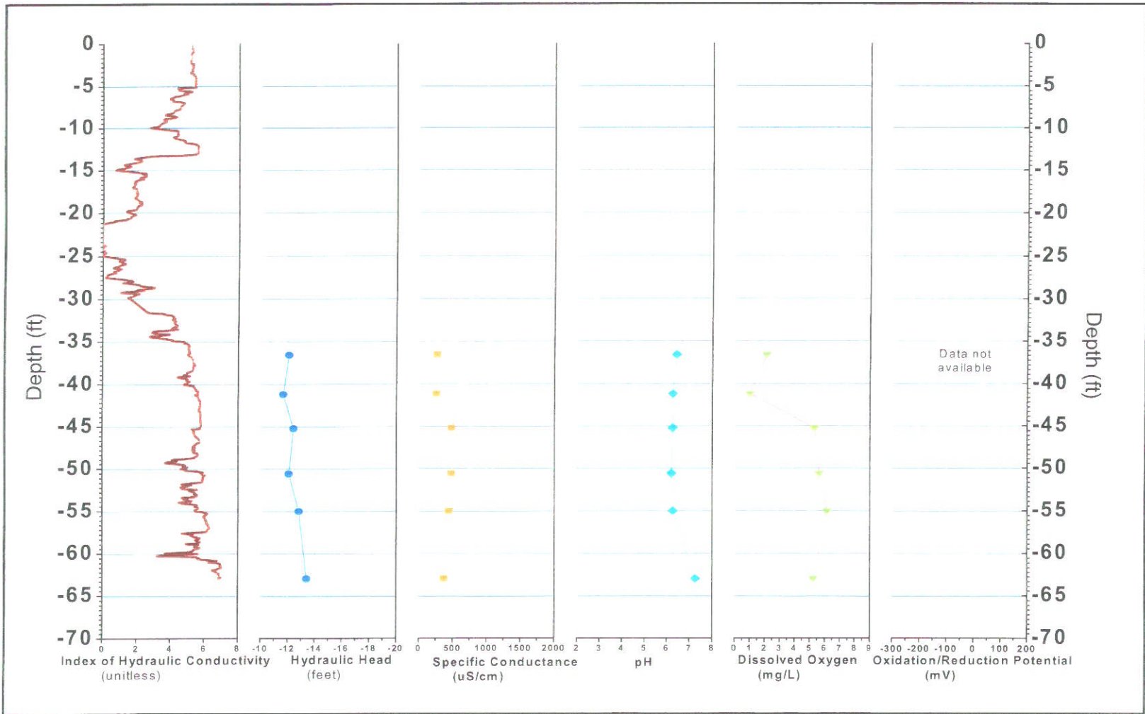
FIGURE B-240, I_k RECORD AND PHYSICO-CHEMICAL PARAMETERS ERM, Wayland, Massachusetts
