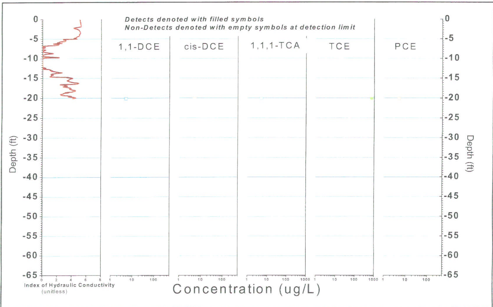
FIGURE B242, I K RECORD AND SELECTED VOC ANALYTICAL RESULTS ERM, Wayland, Massachusetts
