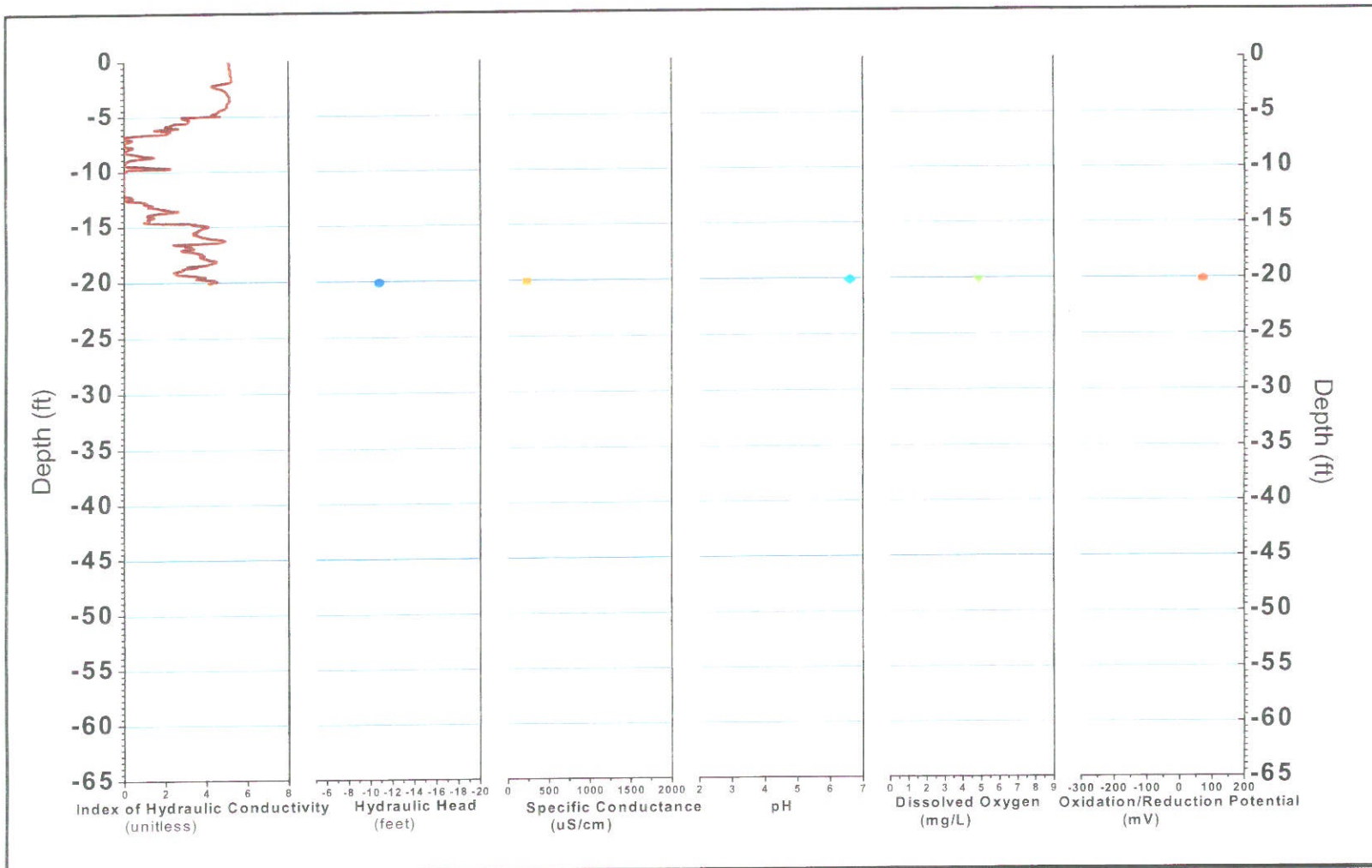
FIGURE B-242, I k RECORD AND PHYSICO-CHEMICAL PARAMETERS ERM, Wayland, Massachusetts
